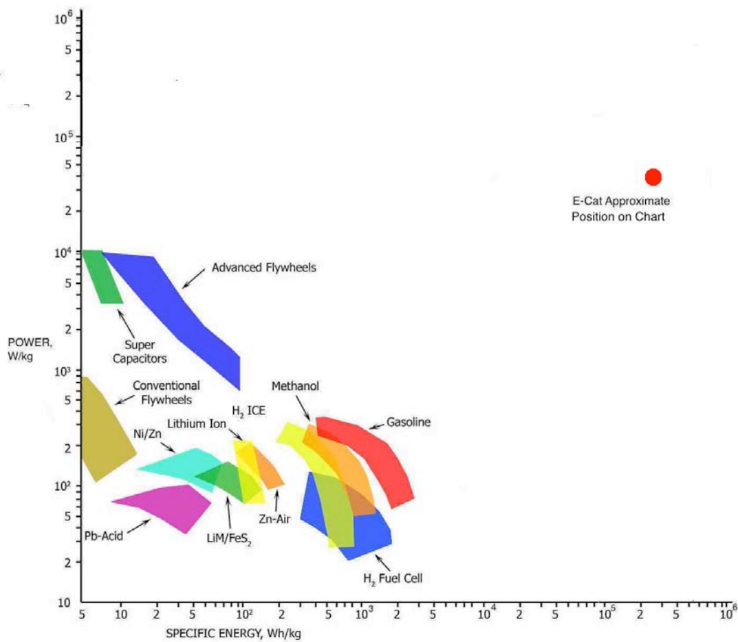
Ragone Plot of Energy Storage
